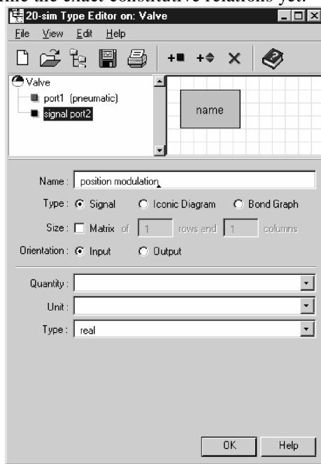
Figure 20: Definition of ports in 20-sim
