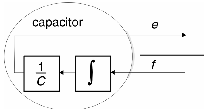
Figure 11: Preferred integral causality of a capacitor
