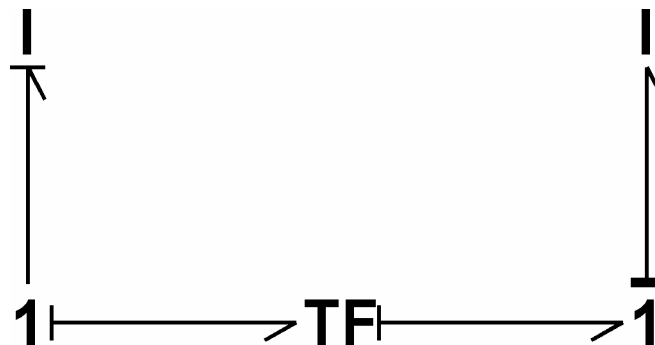
Figure 13: Dependent inertia's via de causal constraints of 1-junctions and transformer
