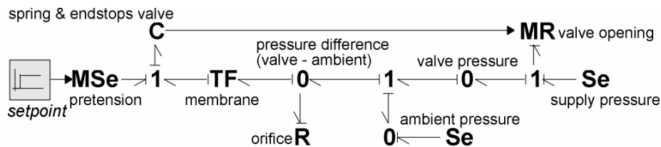
Figure 22: Addition of boundary conditions, flow resistor and structural details (pressures)
