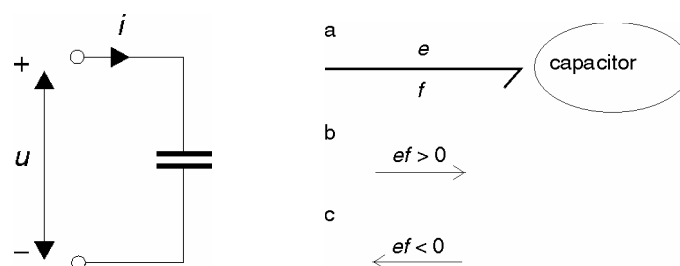
Figure 6: Positive orientation represented by a half arrow, direction depends on sign (b,c)
