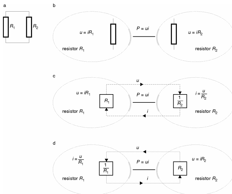
Figure 15: Arbitrary causality of two resistors causing an algebraic loop
