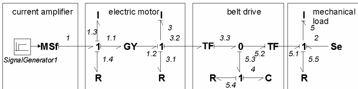
Figure 17: Simple, linear bond graph model of the servo system in figure 16
