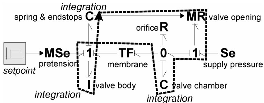
Figure 26: Third order loop (three integrations) via a causal path and the modulation signal
