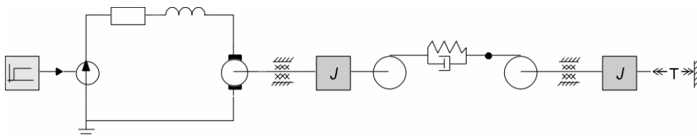
Figure 16: Iconic representation of a servo system with belt drive (graphical 20-sim input)
