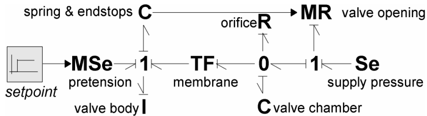
Figure 25: Addition of the compressibility of the air in the valve chamber (C)
