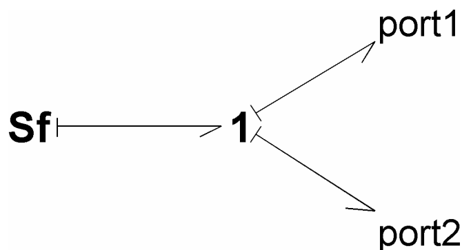
Figure 12: Propagation of a fixed causality via a 1-junction
