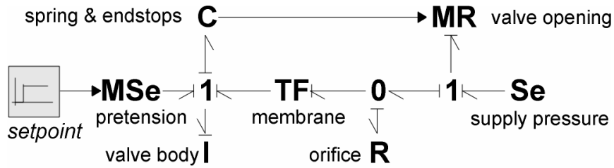
Figure 24: Addition of the valve body mass
