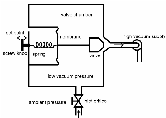
Figure 18: Sketch of the low-vacuum control valve
