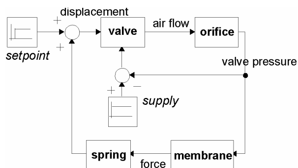
Figure 19: Algebraic model resulting from functional description
