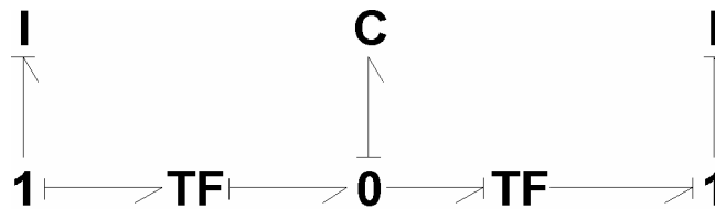
Figure 14: Independent inertia's by adding the elasticity of the transmission (e.g. belt-drive)
