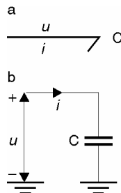
Figure 8: Bond graph representation of an electrical capacitor
