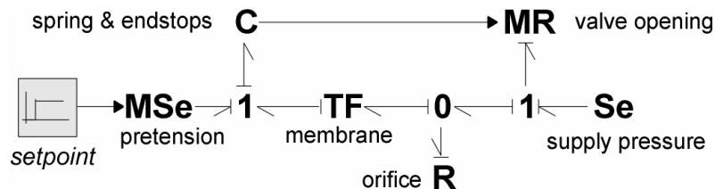
Figure 23: Simplification by choosing ambient pressure as reference pressure
