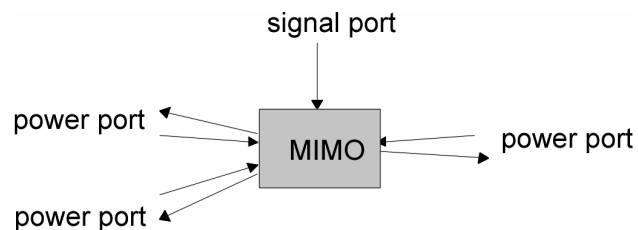
Figure 4b : MIMO system with bilateral power ports and modulating signal ports
