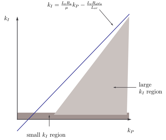
Fig. 2. Stability regions in the gains space. The height of the small k_I region may actually vary with k_P .
