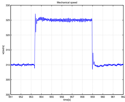
Fig. 6. Experimental results: mechanical speed w .
