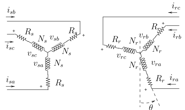
Fig. 2. Basic scheme of the doubly-fed induction machine.
